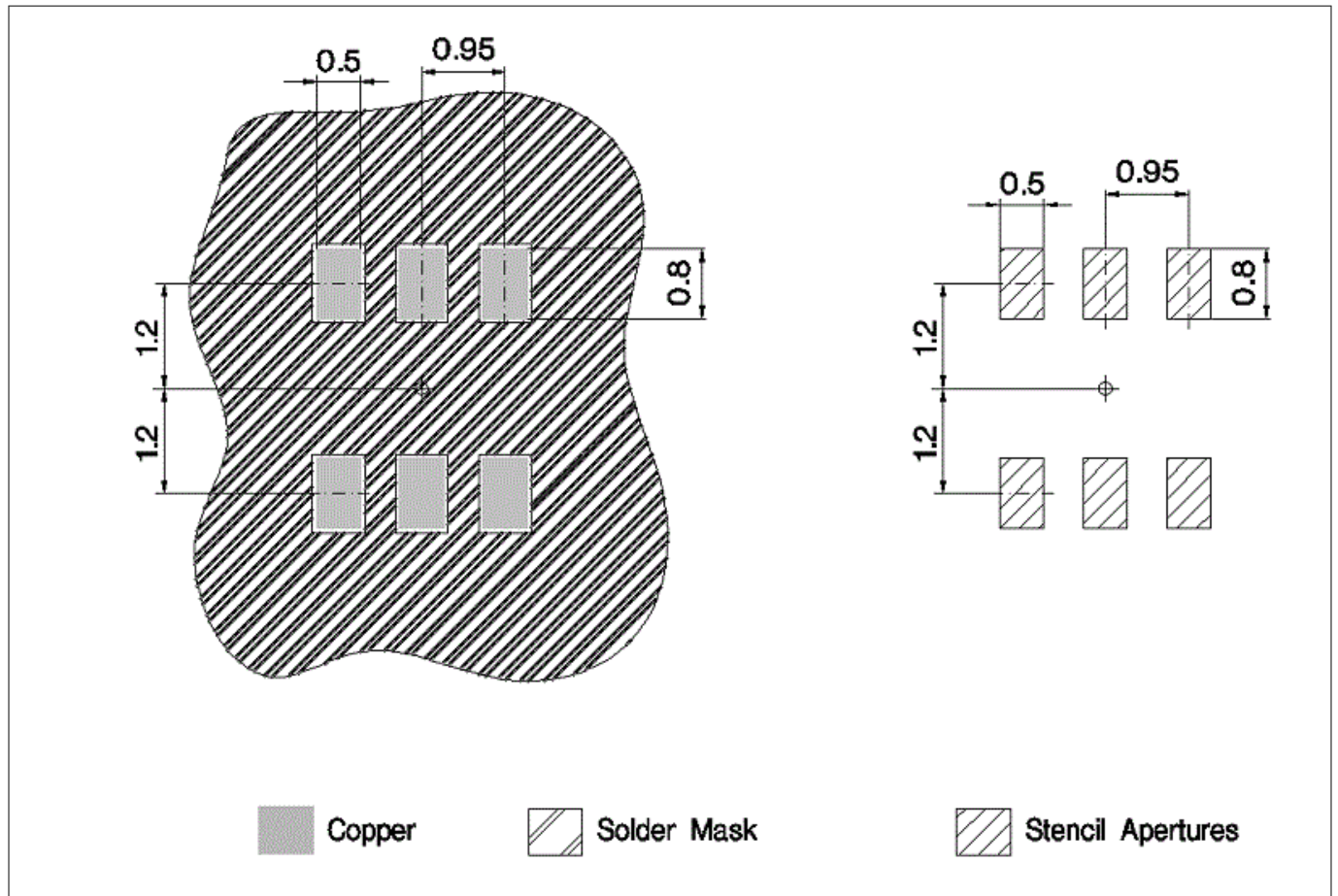
Figure 6 Footprint
